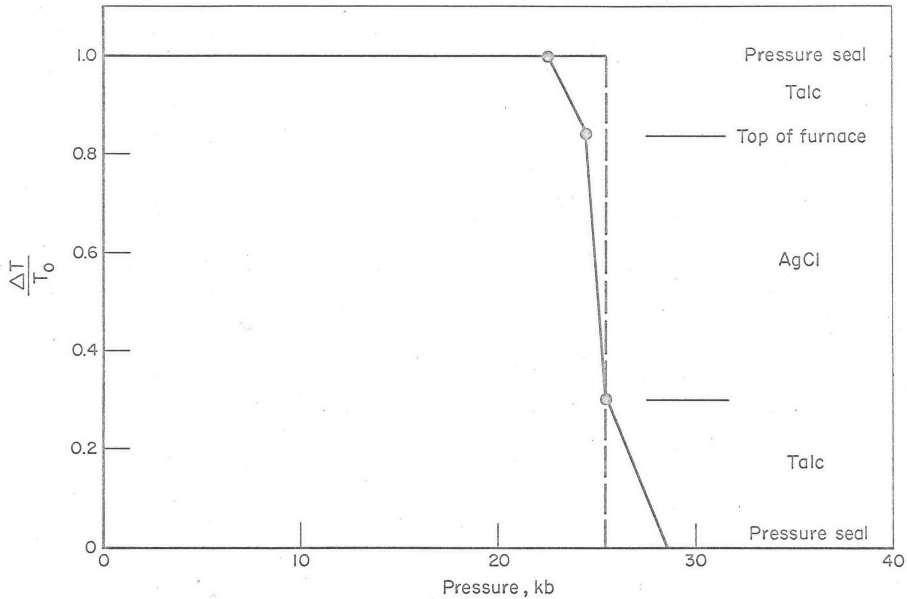
PRESSURE-TEMPERATURE RELATION
